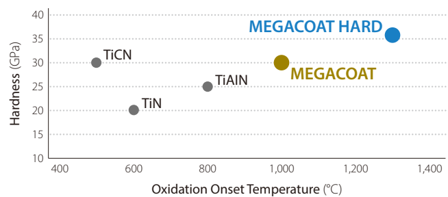
Coating Properties (Comparison with our conventional grade)
